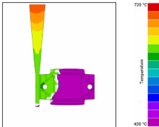
Figure 5: Temperature contours showing the position of the pyrolytic zone after 10 seconds (ProCAST).
