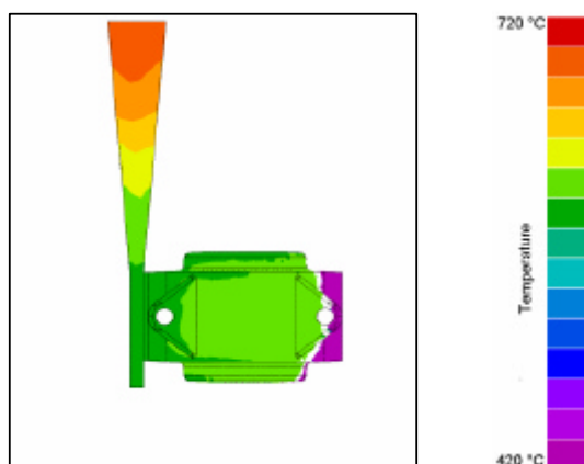
Figure 7: Temperature contours showing the position of the pyrolytic zone after 12.8 seconds (ProCAST).
