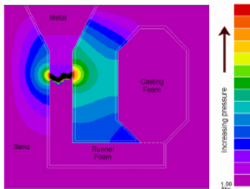
Figure 2: (left) Pressure contours after 1.0 second. The pressure contours, caused by the formation of gas, follow the movement of the pyrolytic zone (ProCAST).
