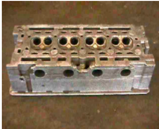
Figure 11: Montupet designed and used a 4 slice prototype cylinder head as a research part (Courtesy of Montupet).
