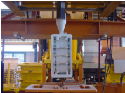
Figure 9: (left) The coated foam just before the vibration station. (Courtesy of Montupet)
