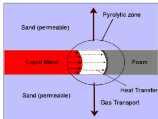
Figure 1: The figure shows a simplified representation of the pyrolytic zone where the metal is advancing and the foam is progressively disappearing through pyrolysis.
