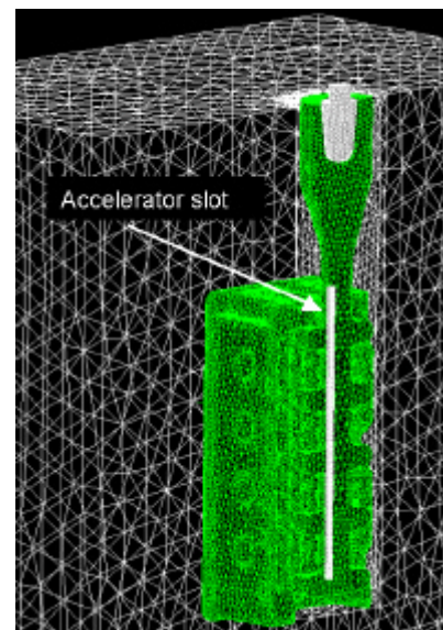
Figure 12: (right) The Finite Element mesh of an industrial lost foam casting of a cylinder head component. (ProCAST).
